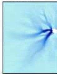
(f) Narrow, topographically constrained trunk at the downstream end; broad onset zone
