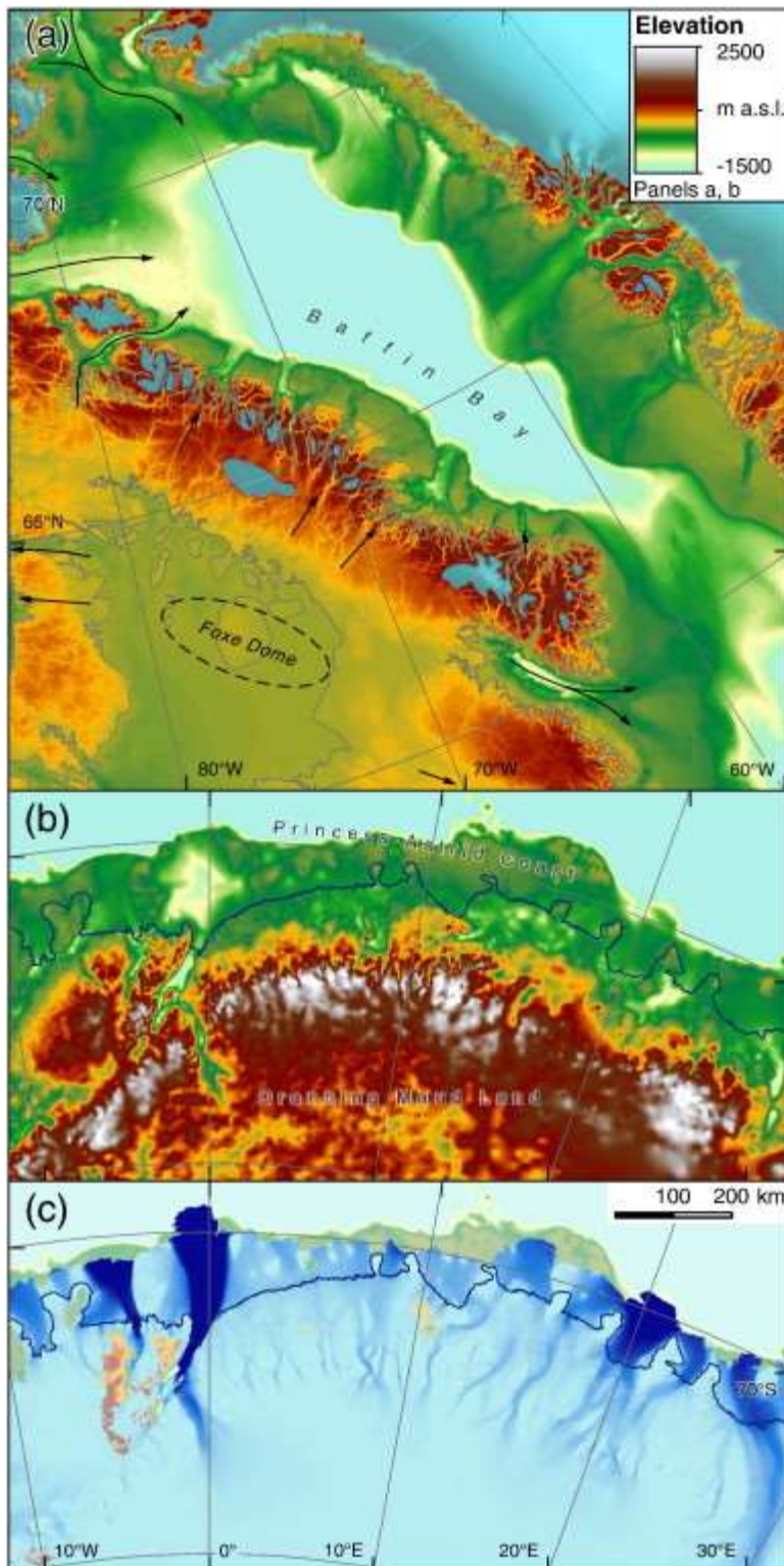
Fig. 7. High-relief coasts modified by selective linear erosion under ice sheet glaciation. (a) Topographic map of Foxe Basin, Baffin Island and Baffin Bay (IBCAO data from Jakobsson et al., 2000 ; location marked in Fig. 3 ). Glacial
