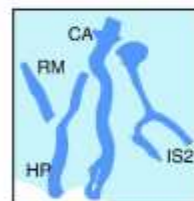
(i) Terrestrial ice streams with a convergent onset zone and a narrow, winding trunk
