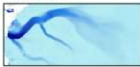
(a) Dendritic simple; long tributaries; flame-like onset Recovery Glacier
