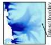
(b) Dendritic; short and wide tributaries Pine Island Gl.
