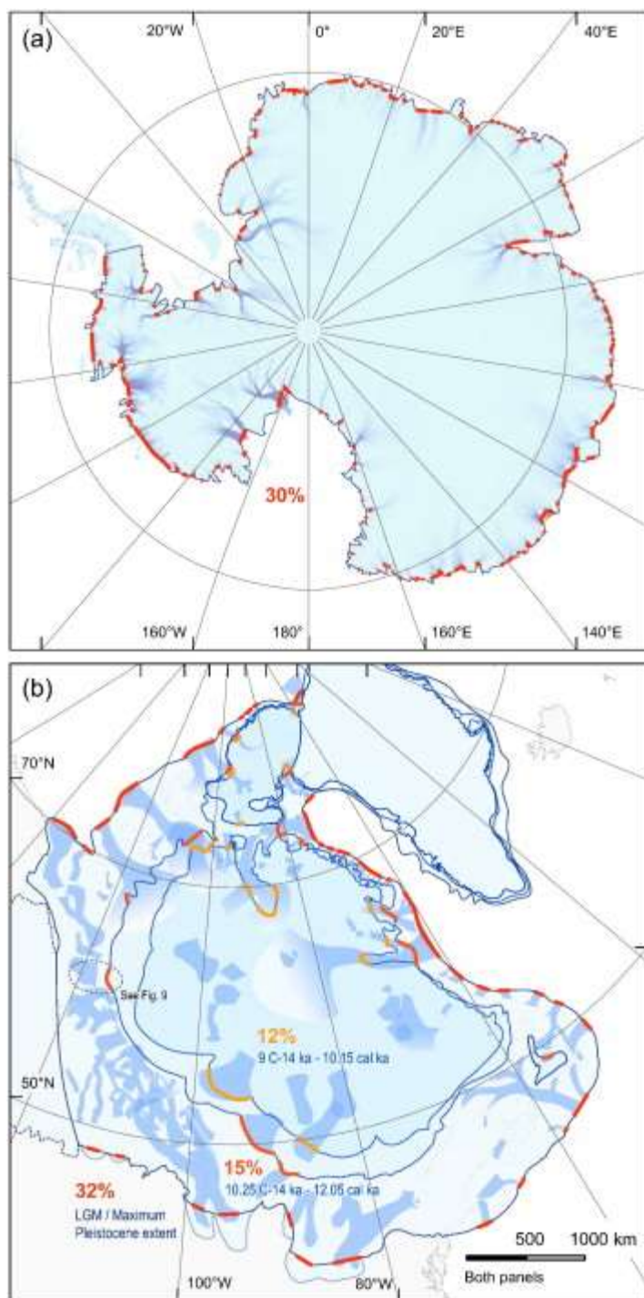
Fig. 20. Percentage of the streaming margin calculated for Antarctica (a) and the Laurentide Ice Sheet (b), using the definition of an ice stream as spatial partitioning of ice flow (see Section 3 ). Streaming margin was mapped manually for Antarctica from data by Rignot et al. (2011c) and ice streams reconstructed by Margold et al. (2015) were used for the Laurentide Ice Sheet. The Laurentide ice margin is
